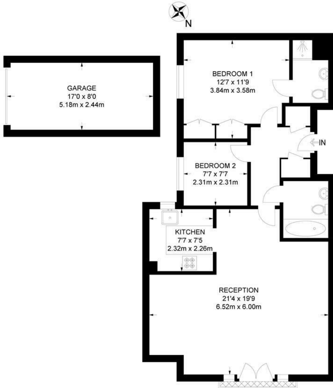
THIRD FLOOR
