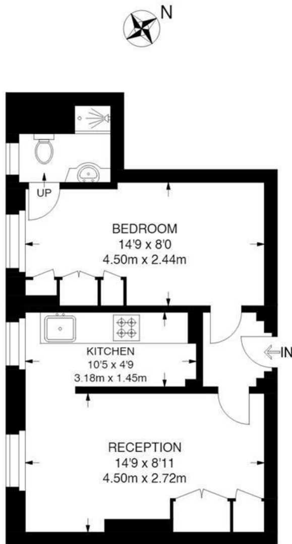
FIRST FLOOR
