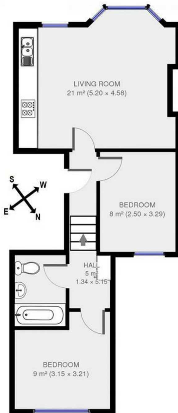
First Floor
