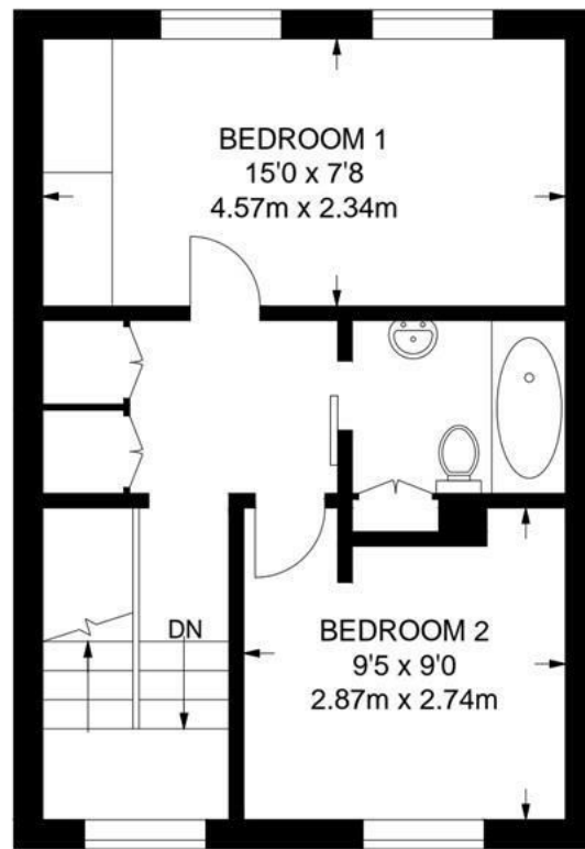
SECOND FLOOR
